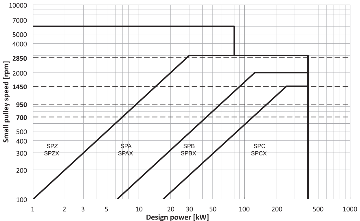
Cross section selection chart for Narrow V-Belts for DIN
