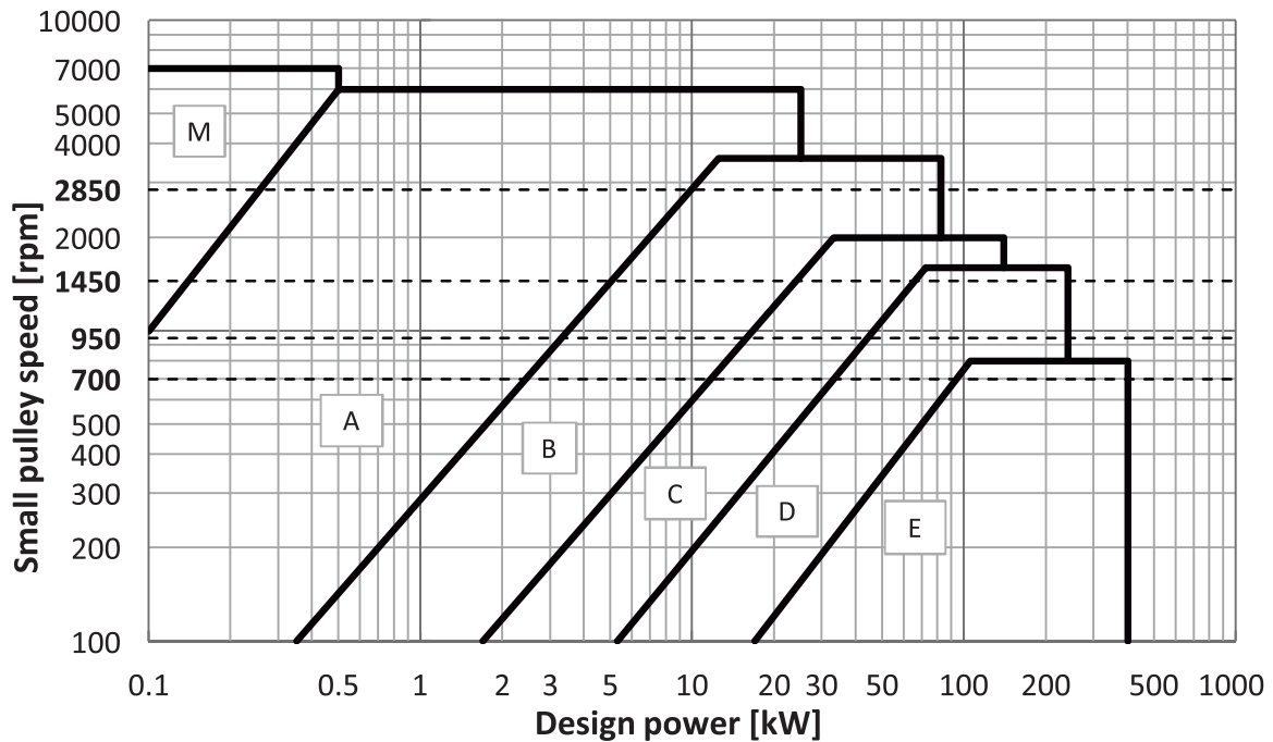
Cross section selection chart for Classical V-Belts for RMA
